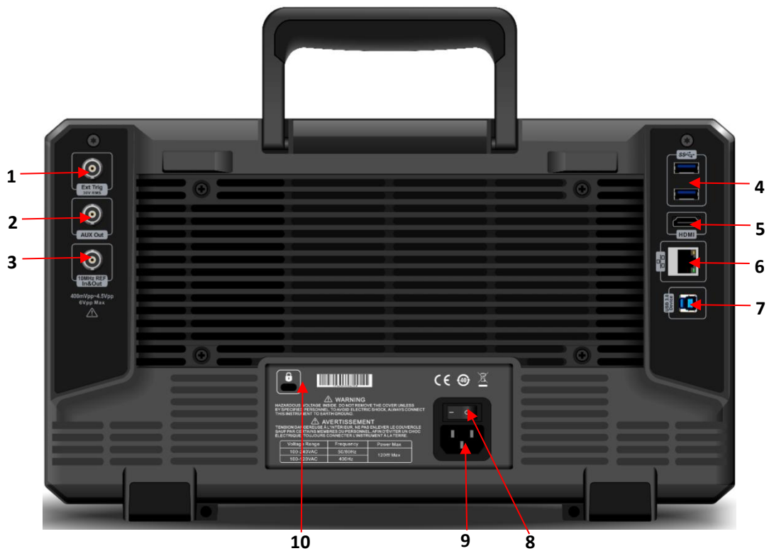
Rear Panel
