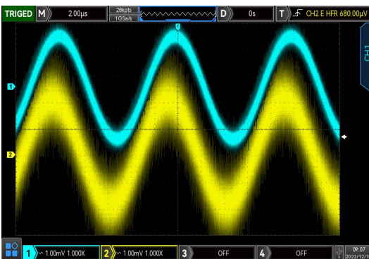
CH1 High SNR @4mV offset DC 2V
