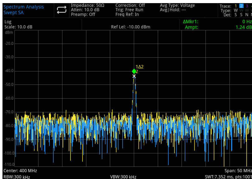
Figure 3-17 Component of Harmonic Distortion
