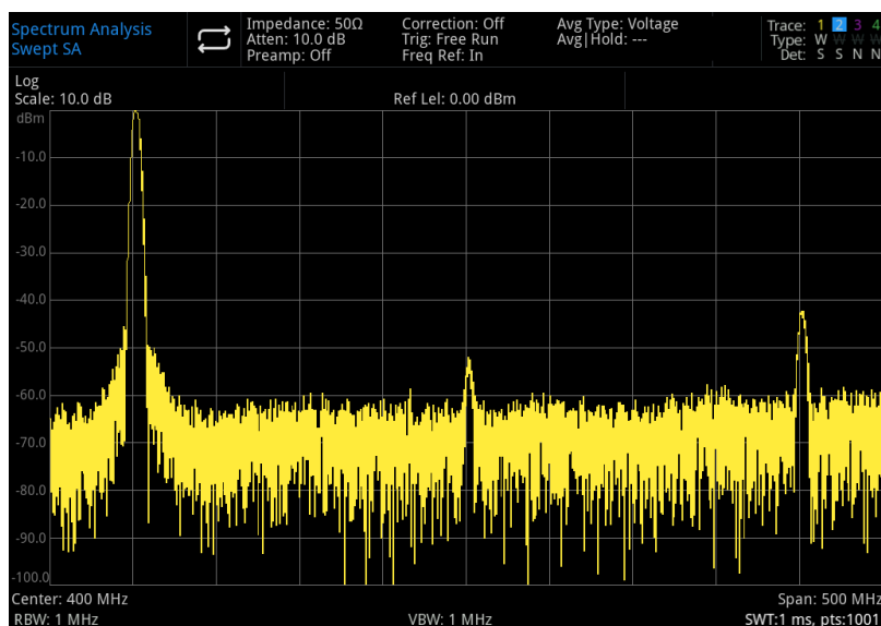
Figure 3-16 Harmonic Distortion
