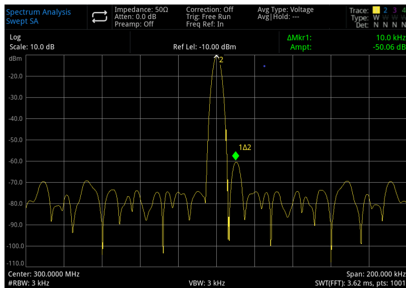
Figure 3-9: Distinguish Small Signal from Big Signal
