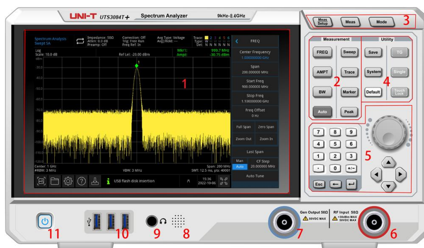
Figure 1-1 Front Panel
