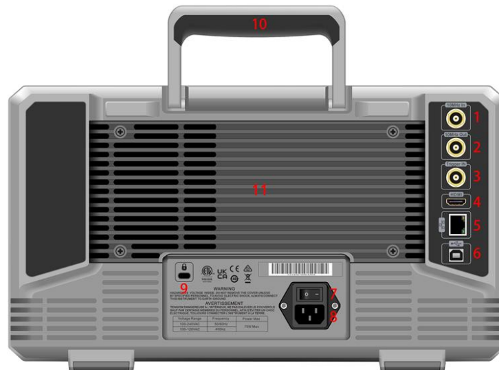
Figure 1-3 Rear Panel
