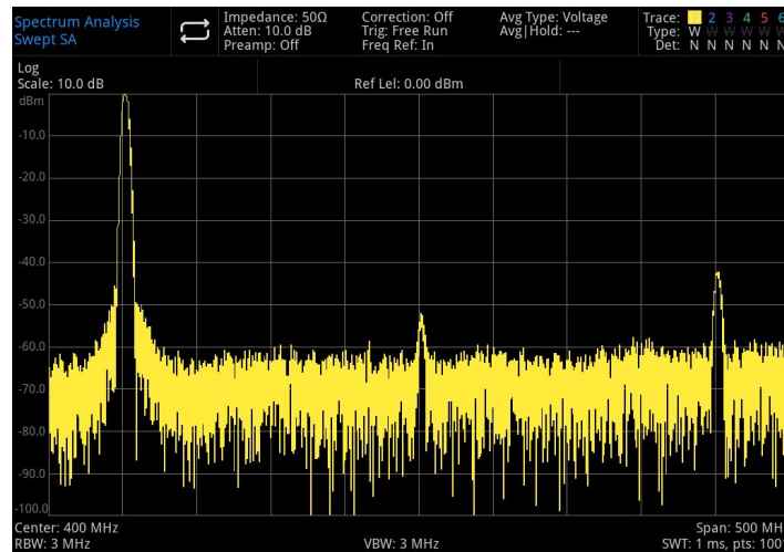
Figure 3-16 Harmonic Distortion
